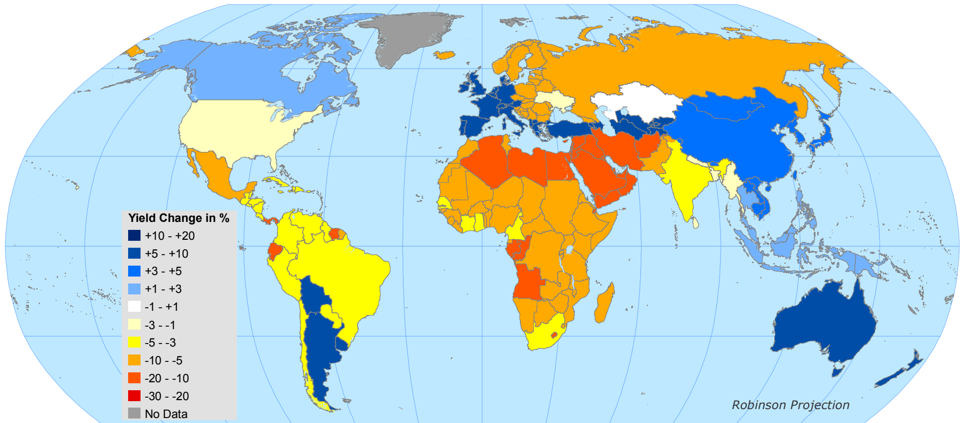
Projected Wheat Yield Change in % 1970-2000 Baseline to 2080, SRES B2B Scenario
